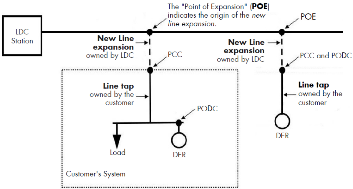
Figure 9: PCC vs PODC (With New Distributor-Owned Line Expansion)
